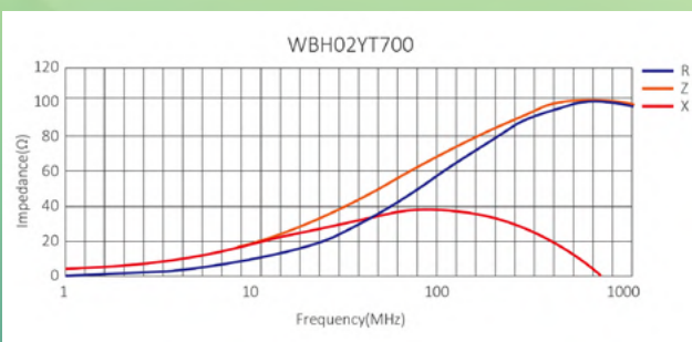
WBH02YT700
