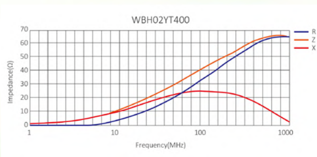
WBH02YT400
