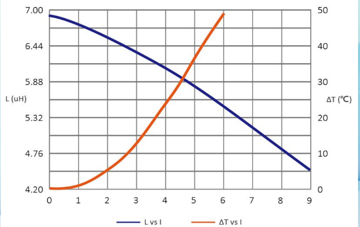
SAR7040MT6R8-M
