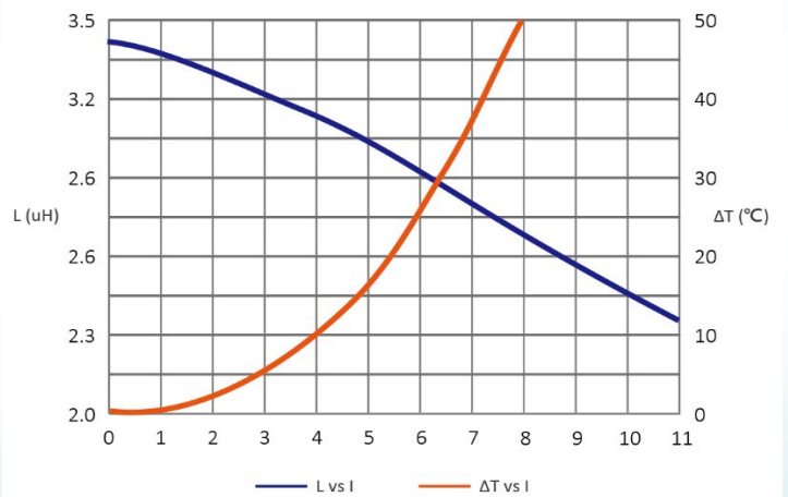
SAR7040MT3R3-M
