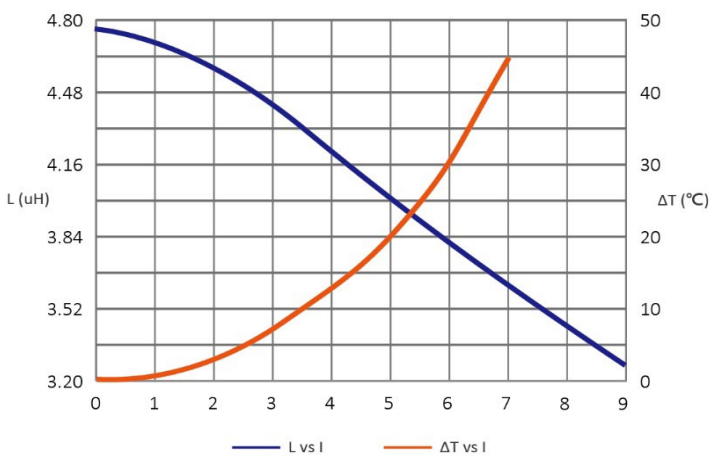
SAR7040MT4R7-M
