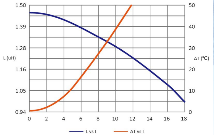
SAR7040MT1R5-M
