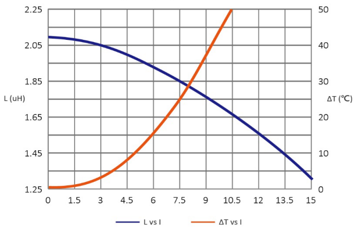
SAR7040MT2R2-M
