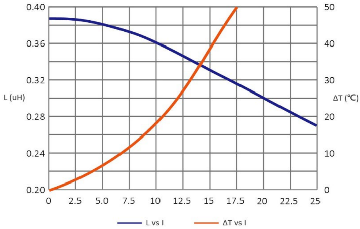
SAR7050MTR36-M
