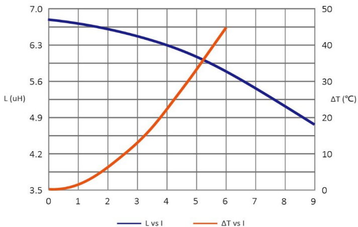
SAR7050MT6R8-M
