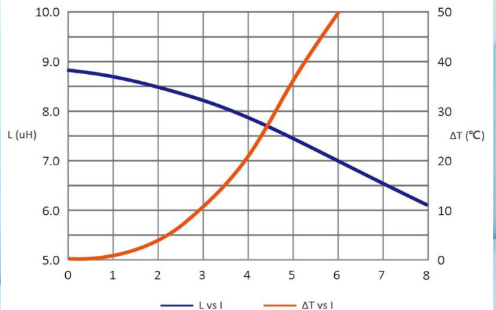
SAR7050MT8R2-M
