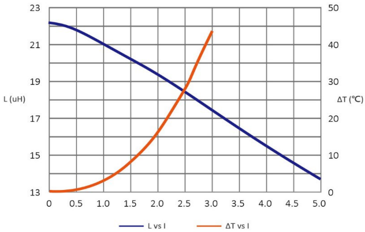
SAR7050MT220-M
