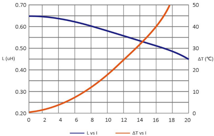
SAR7050MTR68-M
