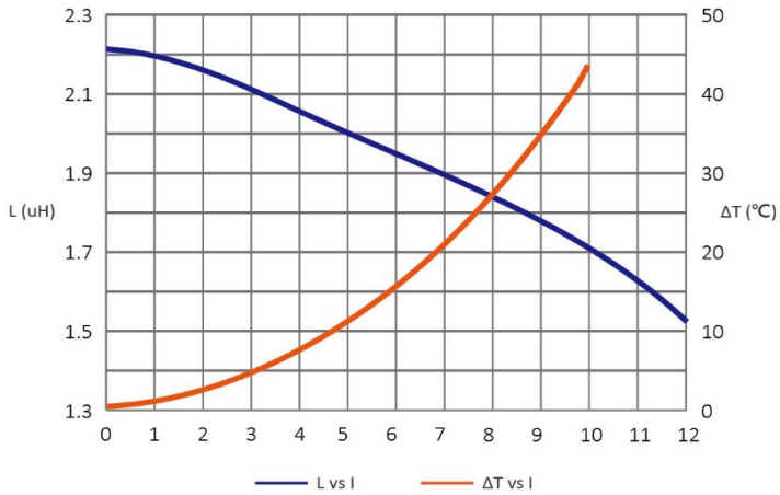
SAR7050MT2R2-M
