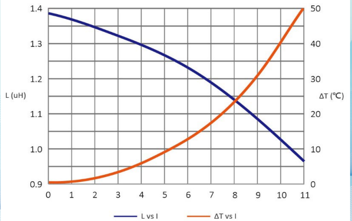
SAR7050MT1R5-M
